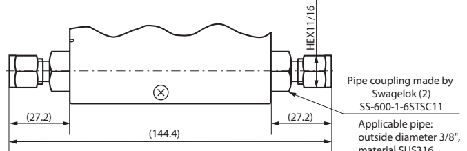
3/8" Swagelok connection type (option)
