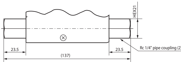
Rc 1/4" connection type (option)
