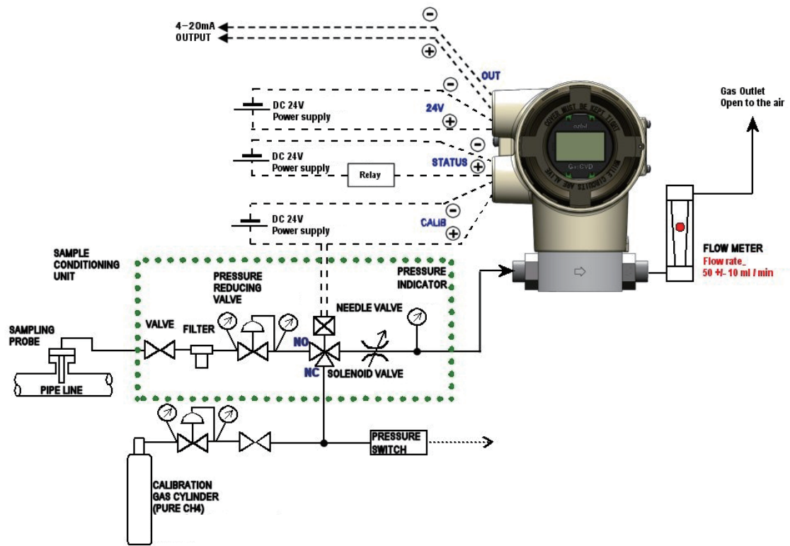
Figure 1. Example of recommended GasCVD installation
