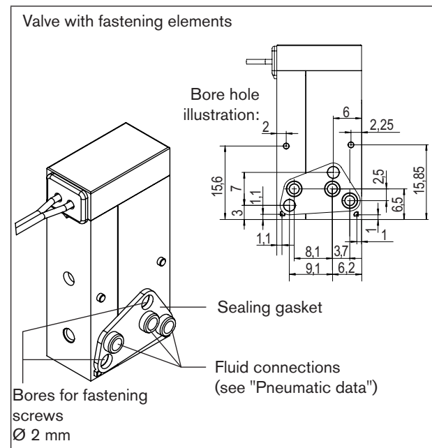
Figure: Assembly drawing
