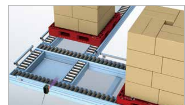
L-shape conveyors (direction converters and loaders) Since detection does not rely on color or material, it is possible to stop objects at the same position.
