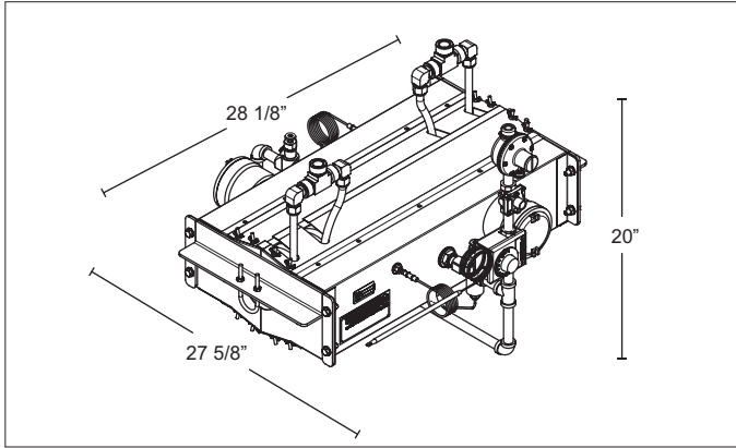
Figure 11 – 6" x 24" Single Coil
