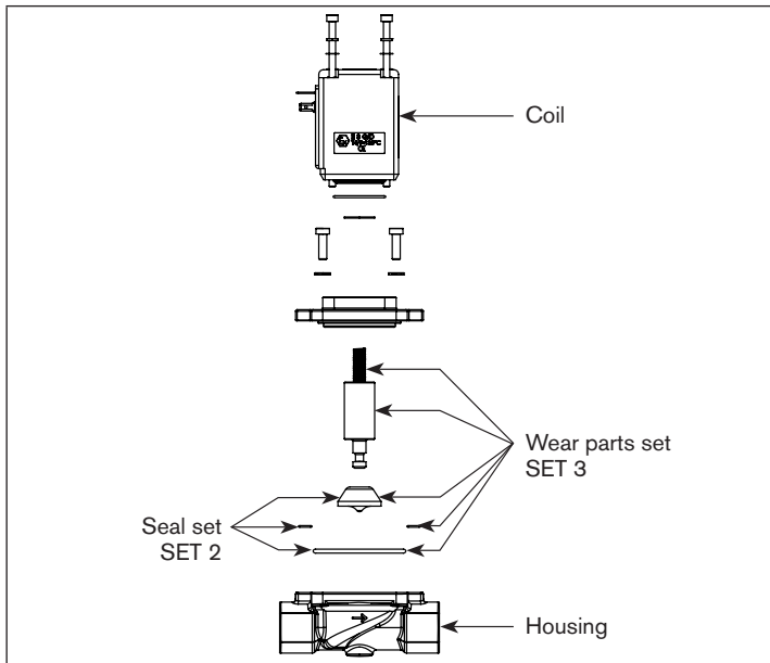
Fig. 5: Overview of replacement spare parts solenoid valve Type 0283
