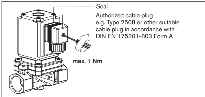
Fig. 4: Connection of the cable plug – example Type 0293
