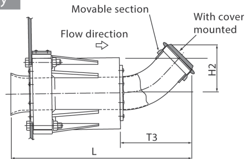
Figure 7. Detector (elbow flange type)
