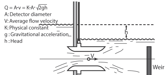
Figure 2. Principle of flow measurement with MagneW3000 Flowmeter
