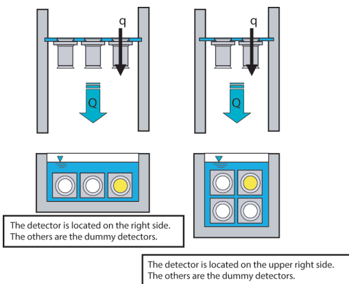
Figure 11. Installation for dummy detector
