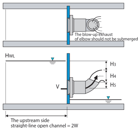
Figure 13. Water head design (Elbow flange method)
