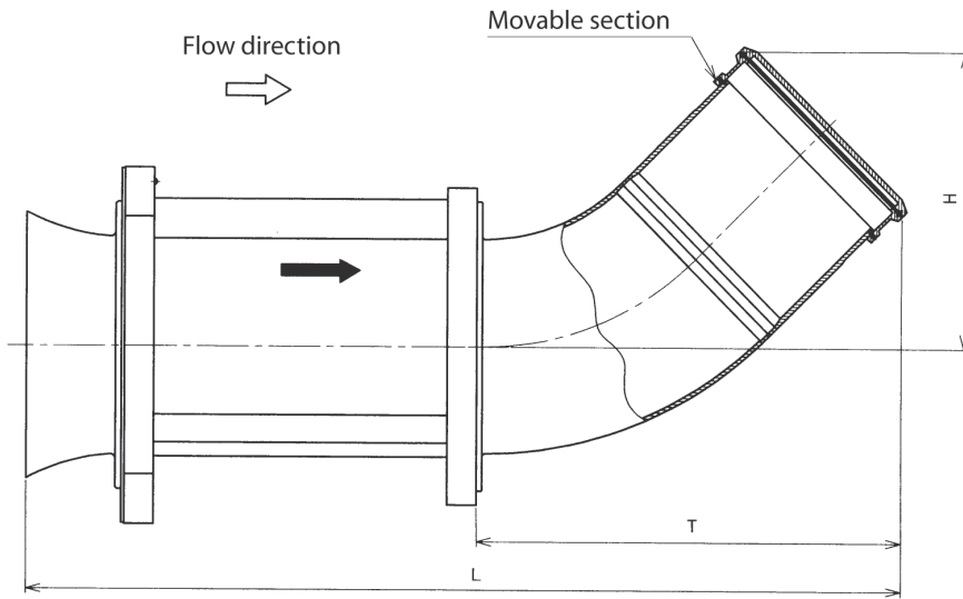
Figure 9. External dimensions (Elbow flange)
