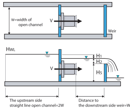
Figure 12. Water head design (Bell mouth type)
