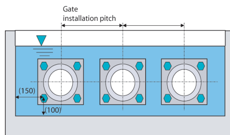
Figure 14. Installation pitch
