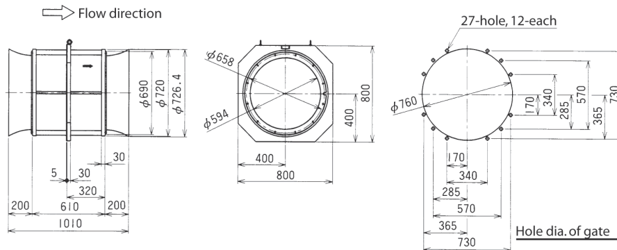
Figure 8. External dimensions (Dummy)
