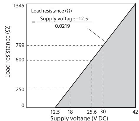
Figure 4. Supply voltage vs. load resistance characteristics
